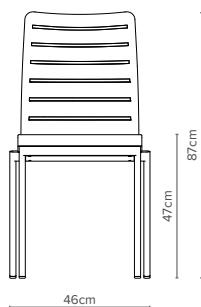
— 08/1 Depth 55.5cm Weight 6.2 kg Stacks up to 10 high
