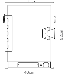
— S.0300 Electric food warmer box Depth 40cm
