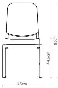
— 66/1 Depth 58cm Weight 5kg Model available as an armchair
